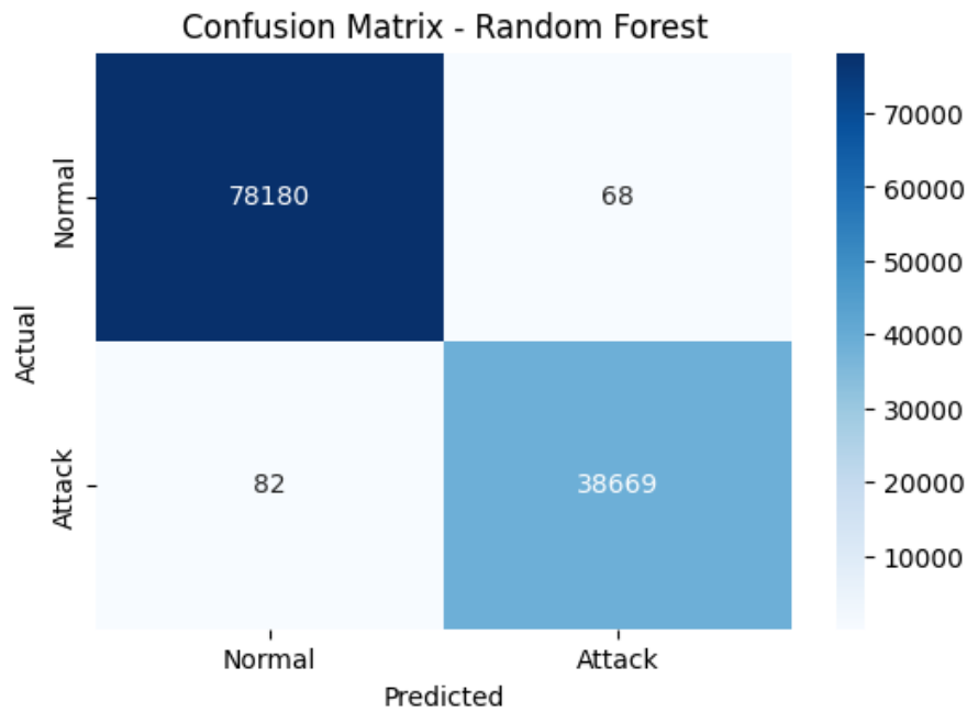
Figure 4: CICIDS2017: Confusion matrix visualization.
