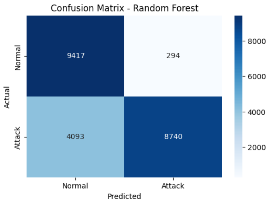
Figure 1: NSL-KDD: Confusion matrix visualization.
