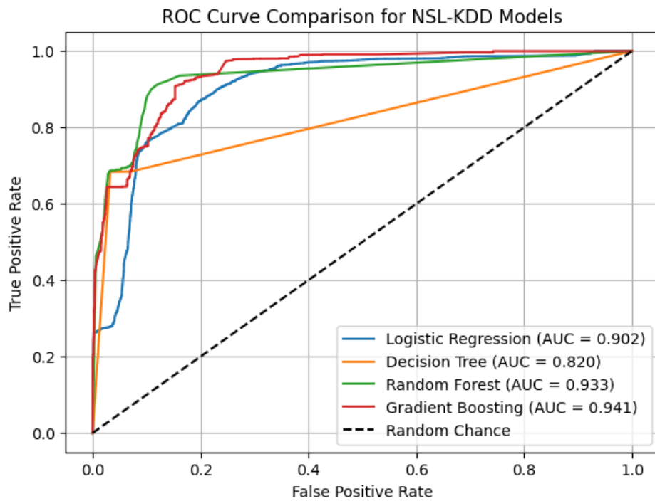
Figure 2: NSL-KDD: ROC curves for all four models.
